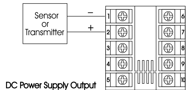
Figure 2-11 Output 2 Wiring
