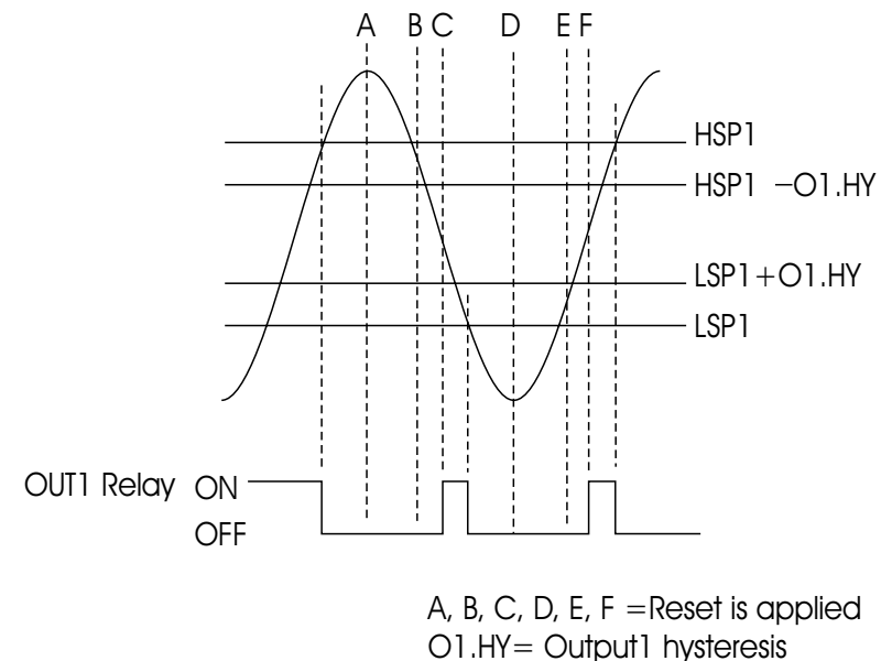
Figure 1-6 High/Low Limit Operation
