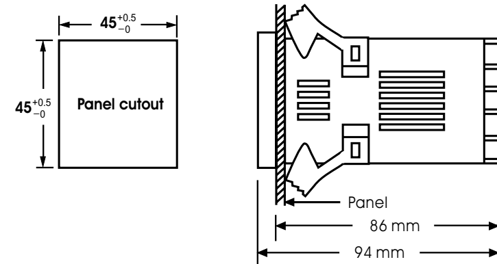
Figure 2-1 Mounting Diagram
